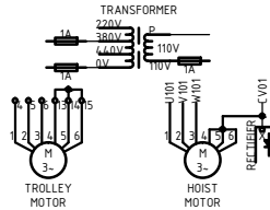
CIRCUIT DIAGRAM OF 380V
