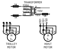
CIRCUIT DIAGRAM OF 220V
