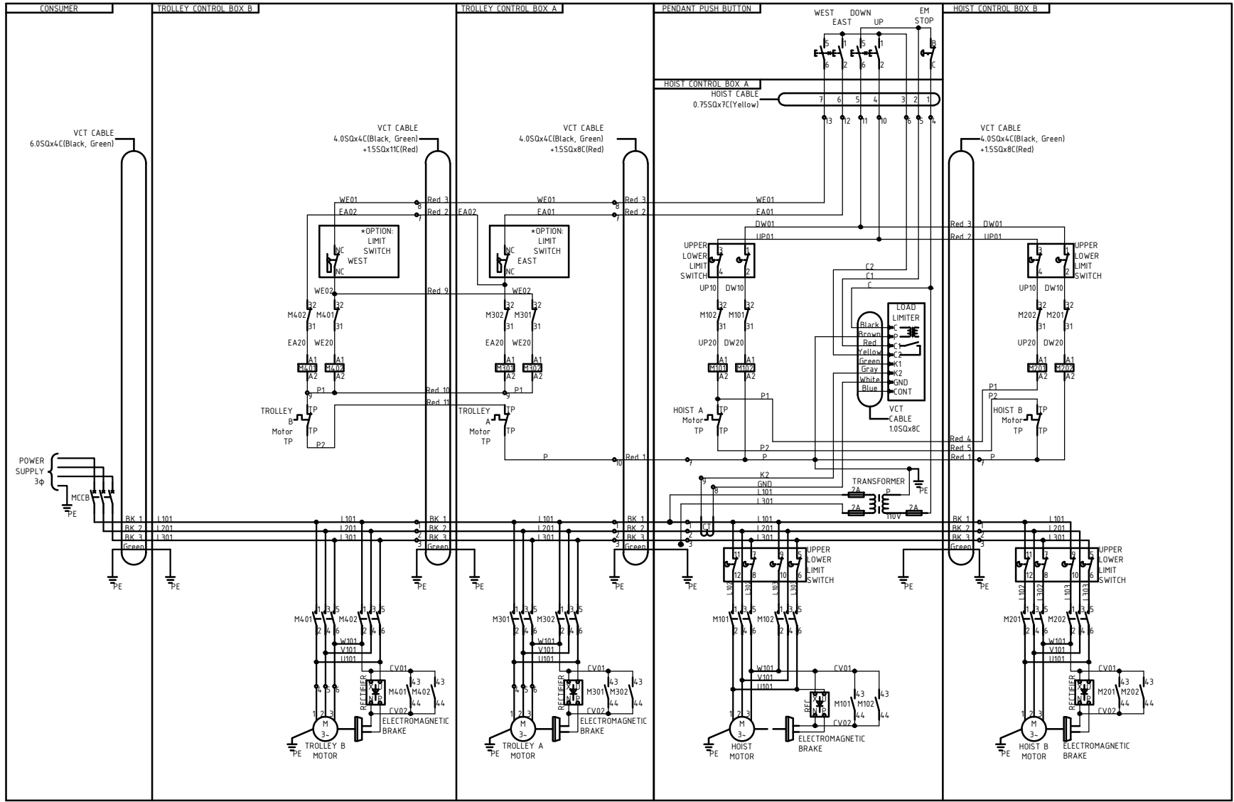
CIRCUIT DIAGRAM OF 440,460,480V
